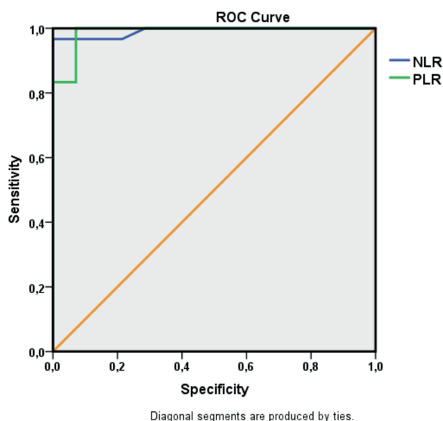
Figure 2. Receiver operating characteristic (ROC) analysis of neutrophil-to-lymphocyte ratio (NLR), platelet-to-lymphocyte ratio (PLR) values for influenza B diagnosis. The figure presents the diagnostic performance and ROC curves of NLR and PLR compared to the control group.
