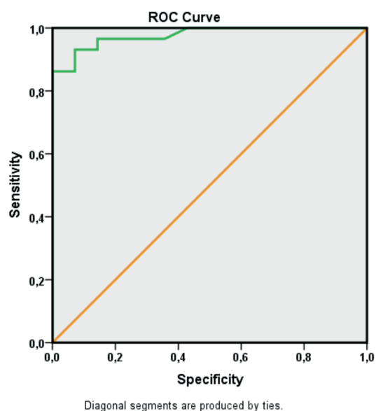
Figure 3. Receiver operating characteristic (ROC) of the Systemic Inflammation Response Index value in influenza B diagnosis. The figure presents the diagnostic performance of SIRI and the ROC curve in comparison with the control group.
